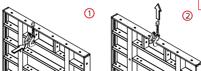
Lifting sling – application
