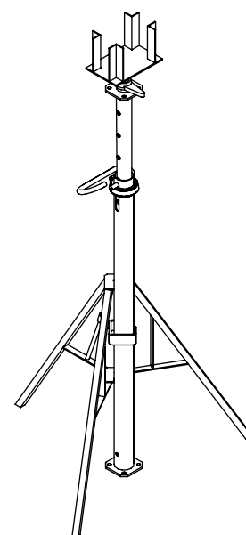
Diagram presenting installation of the support in the tripod
