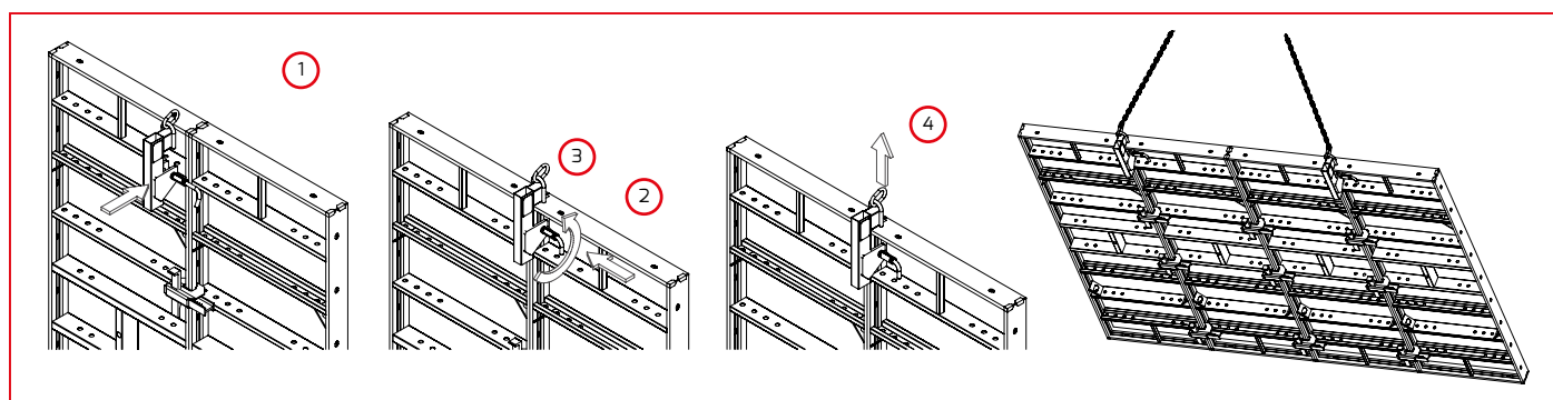
Lifting sling – sample assembly
