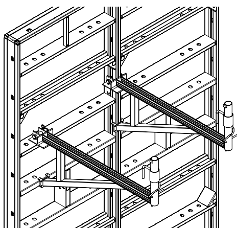
Diagram – working platform assembly
